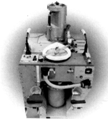
Space Shuttle "unisex" urinal
